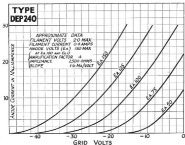
Characteristic Curve of Average DEP 240 Valve.
